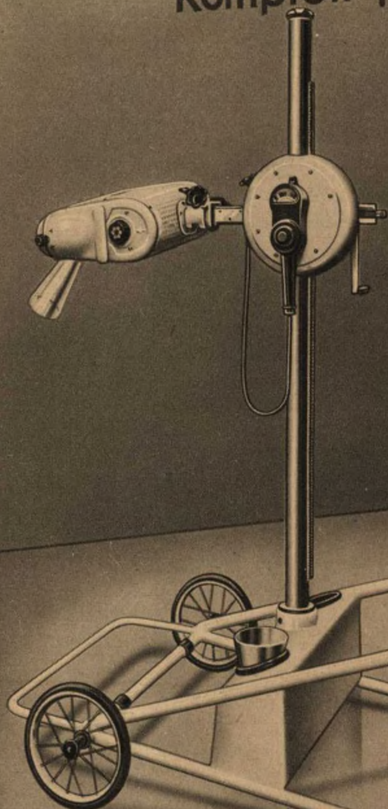
Fahrbare Medixstation
